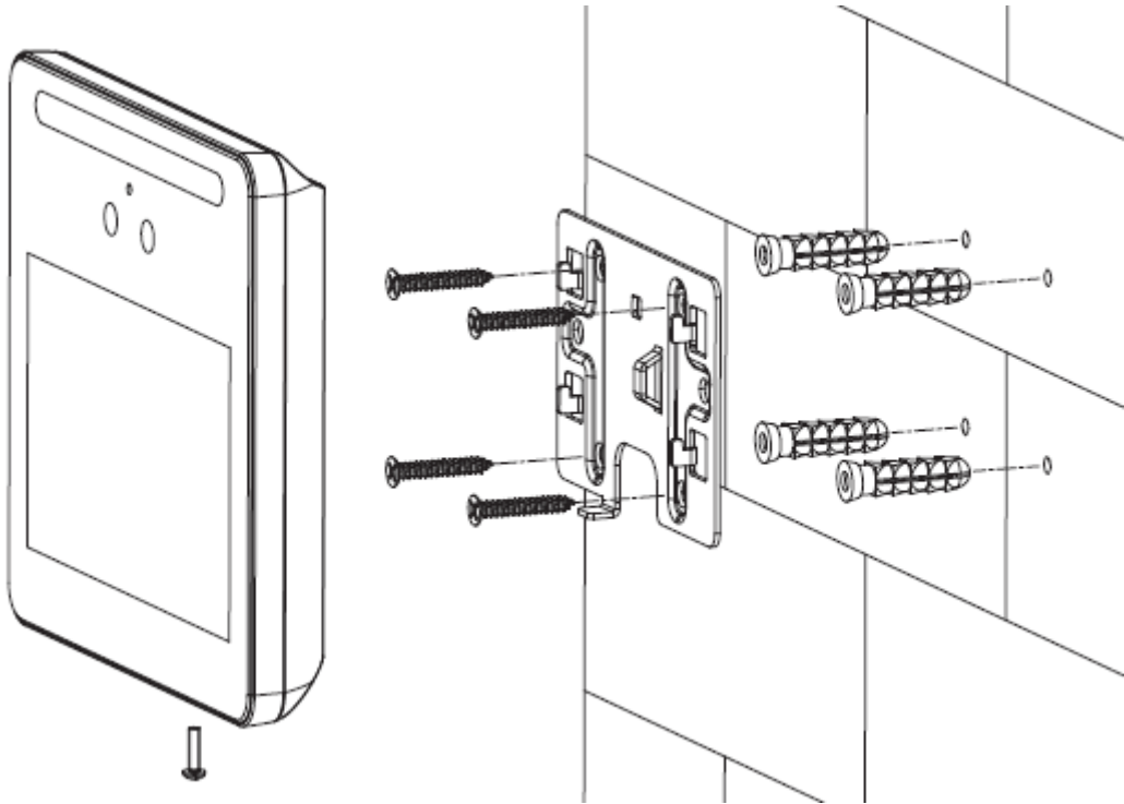
Figure 2-9 Wall installation
