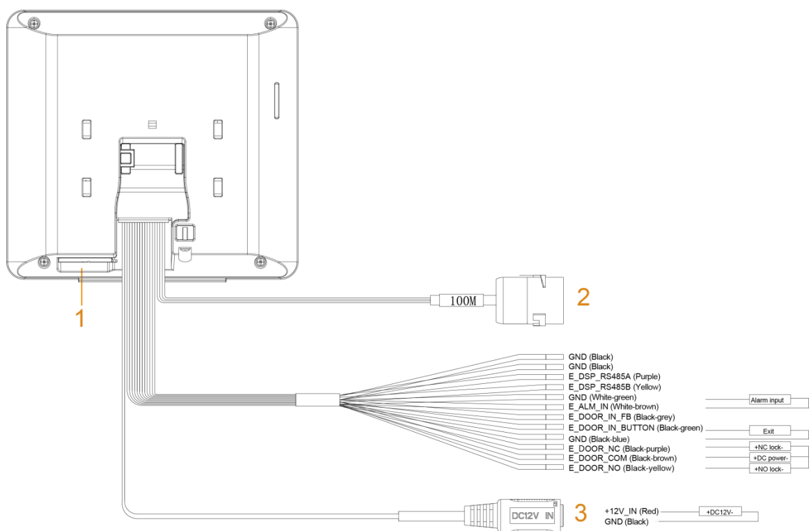
Figure 2-1 Cable connection
